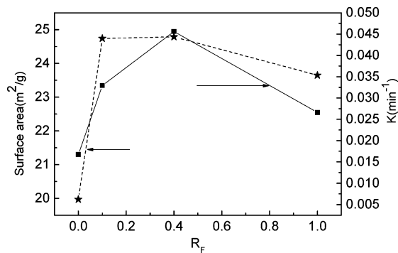
Figure 10. The dependence of the apparent rate constants ( k/\text{min}^{-1} ) and surface areas on fluorine amount for samples at 180 \text{ }^\circ\text{C} for 24 h.
