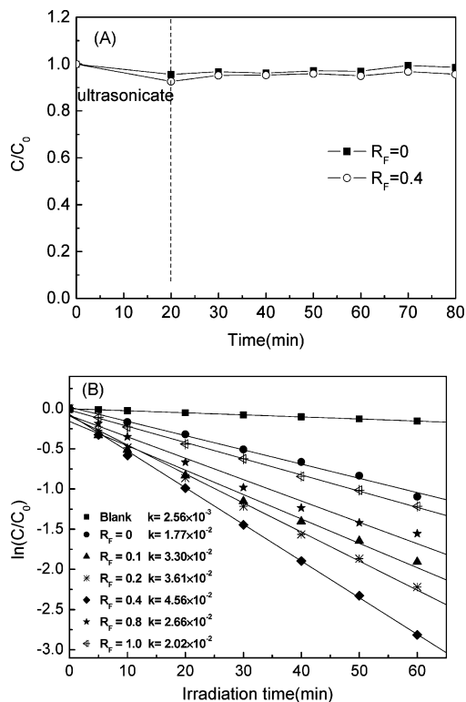
Figure 8. (A) The adsorption of RhB on undoped \text{ZnWO}_4 and doped \text{ZnWO}_4 samples in the dark are compared. (B) The photocatalytic activities of various samples with different amounts of doped fluorine, catalyst loading, 0.50 \text{ g L}^{-1} ; RhB, 1.0 \times 10^{-5} \text{ mol L}^{-1} .
