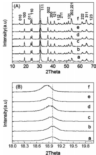
Figure 1. (A) XRD patterns of the samples prepared from NH 4 F–H 2 O mixed solution with different R_F values at 180 °C for 24 h. (a) 0, (b) 0.1, (c) 0.2, (d) 0.4, (e) 0.8, (f) 1.0. (B) Diffraction peak positions of the (100) plane in the range of 2\theta = 18\text{--}20^\circ .
