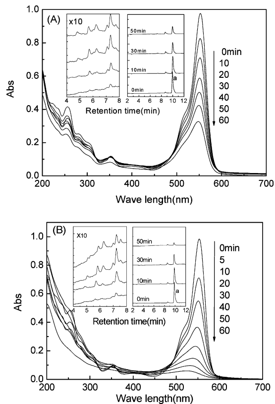
Figure 9. Temporal evolution of the spectral changes during the photodegradation of RhB over \text{ZnWO}_4 with different doped fluorine concentrations and HPLC chromatograms (inset) of RhB solution at various time intervals for the photocatalytic degradation process, (A) R_F = 0 , (B) R_F = 0.4 .
